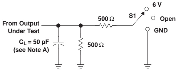
LOAD CIRCUIT
